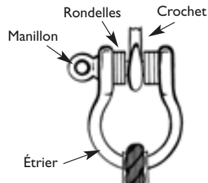
Figure 3.22 Manille stable
