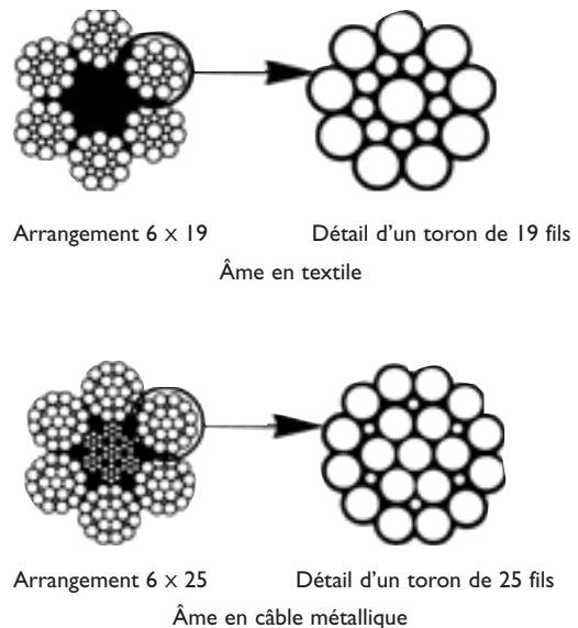
Figure 3.8 Arrangements de câble d'acier
