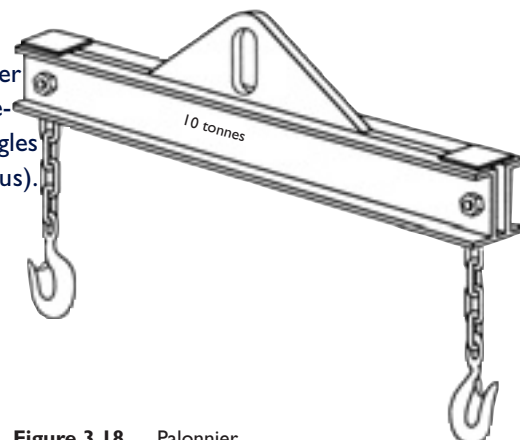
Figure 3.18 Palonnier
